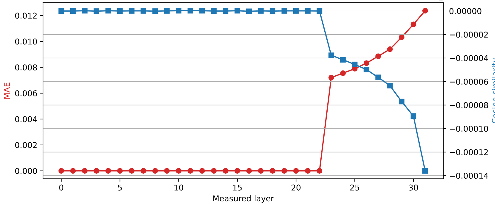
Mistral-7B-Instruct-v0.3 | Quantized layer 22 | float64 → int8
