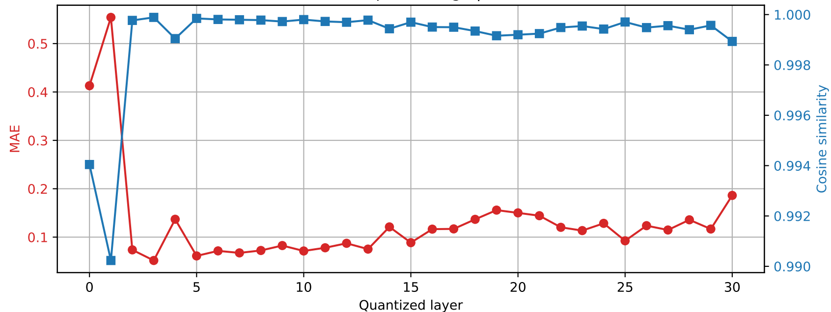
Mistral-7B-Instruct-v0.3 | Prompt 3 Final RMSNorm output damage | float64 → int8
