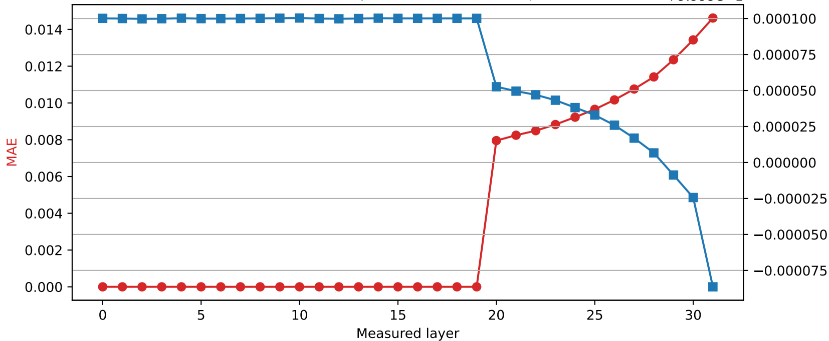
Mistral-7B-Instruct-v0.3 | Quantized layer 19 | float64 \rightarrow int8 +9.999e-1
