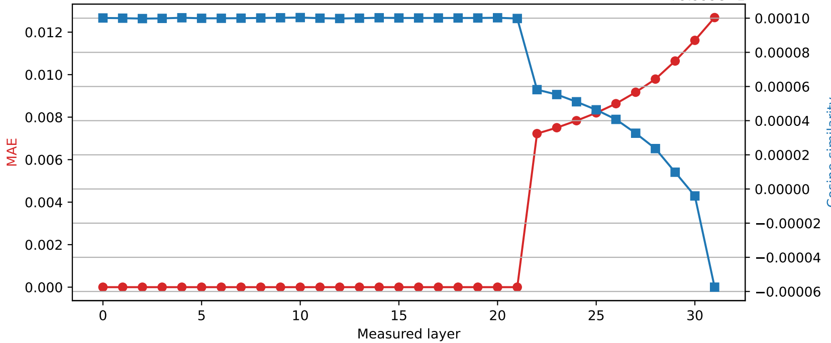
Mistral-7B-Instruct-v0.3 | Quantized layer 21 | float64 → int8 +9.999e-1
