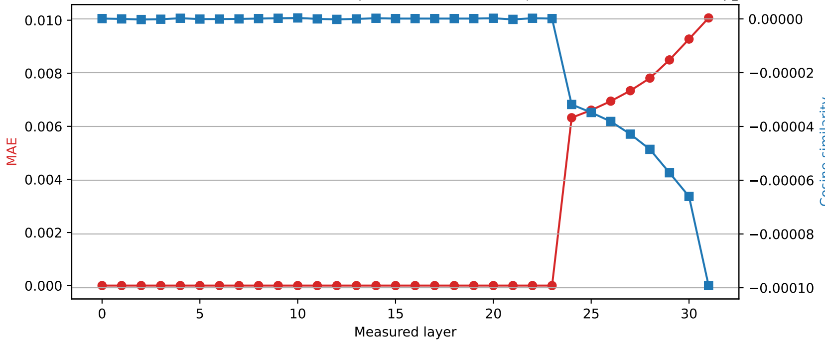
Mistral-7B-Instruct-v0.3 | Quantized layer 23 | float64 → int8
