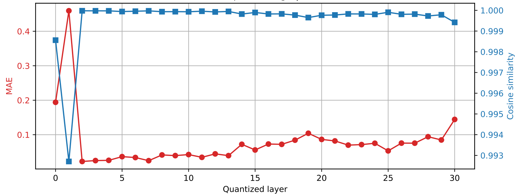
Mistral-7B-Instruct-v0.3 | Prompt 4 Final RMSNorm output damage | float64 → int8
