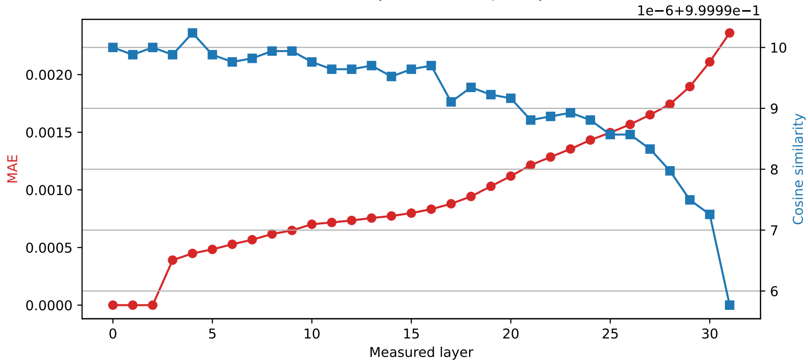
Mistral-7B-Instruct-v0.3 | Quantized layer 2 | float64 → int8
