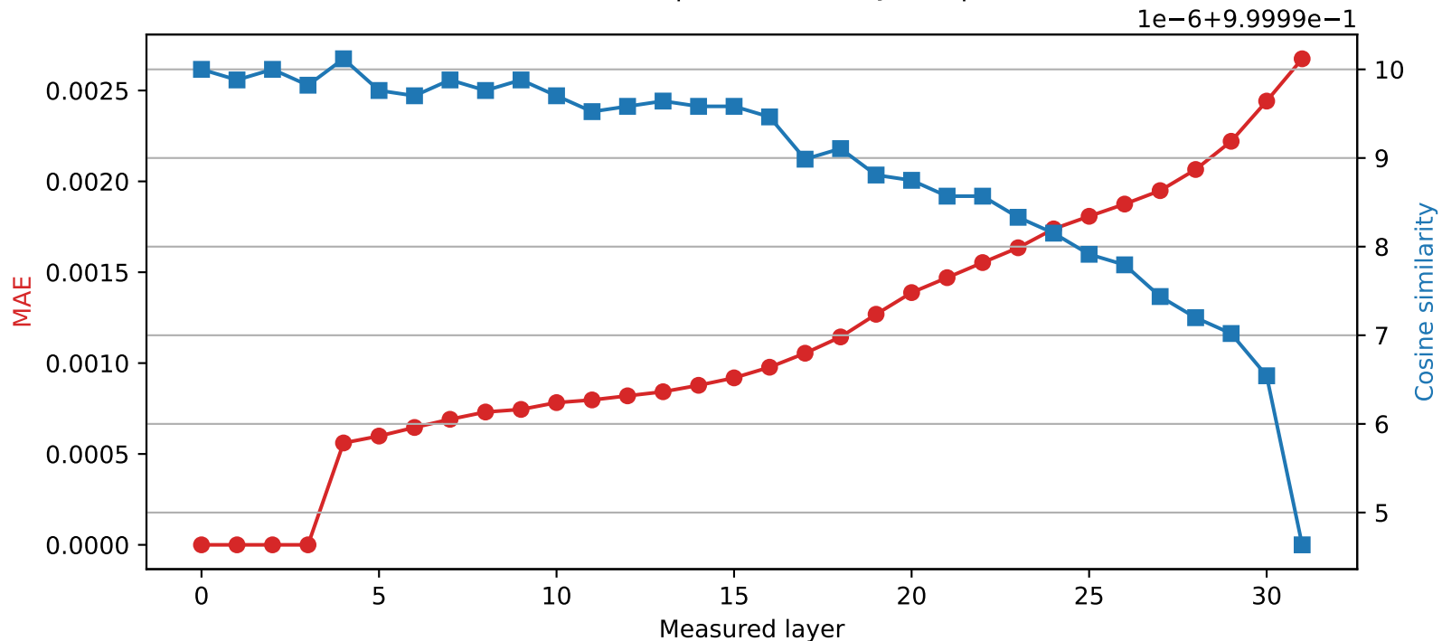
Mistral-7B-Instruct-v0.3 | Quantized layer 3 | float64 → int8
