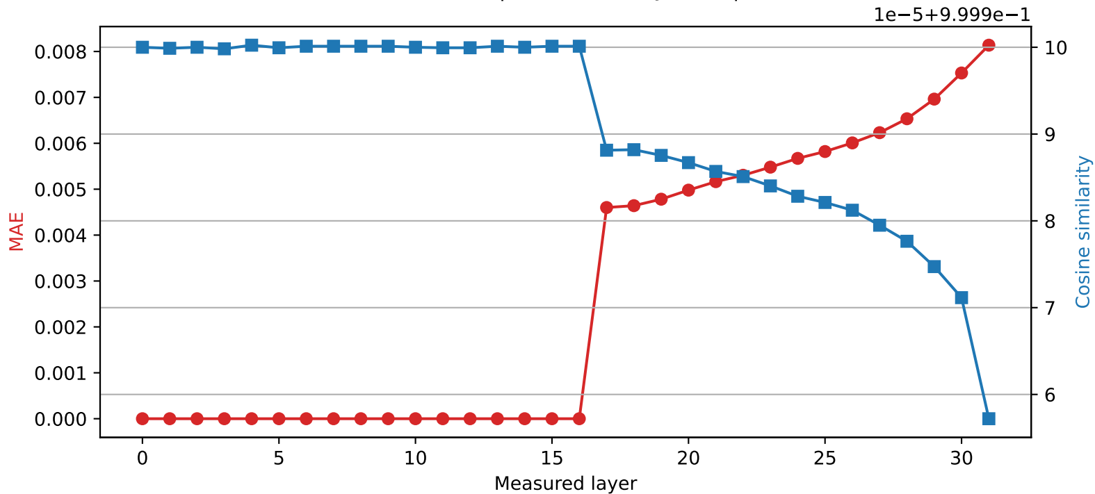
Mistral-7B-Instruct-v0.3 | Quantized layer 16 | float64 → int8
