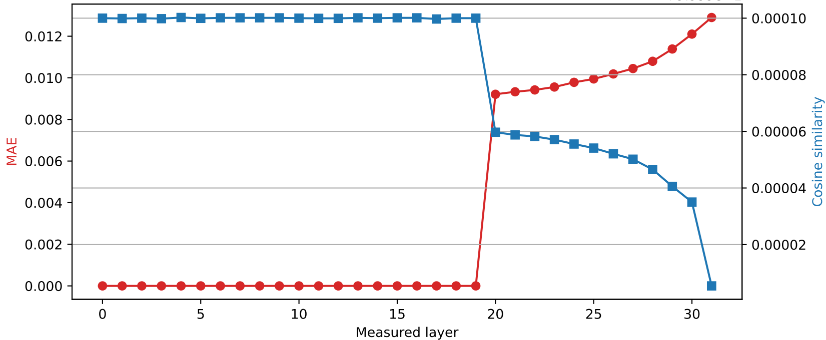
Mistral-7B-Instruct-v0.3 | Quantized layer 19 | float64 → int8 +9.999e-1
