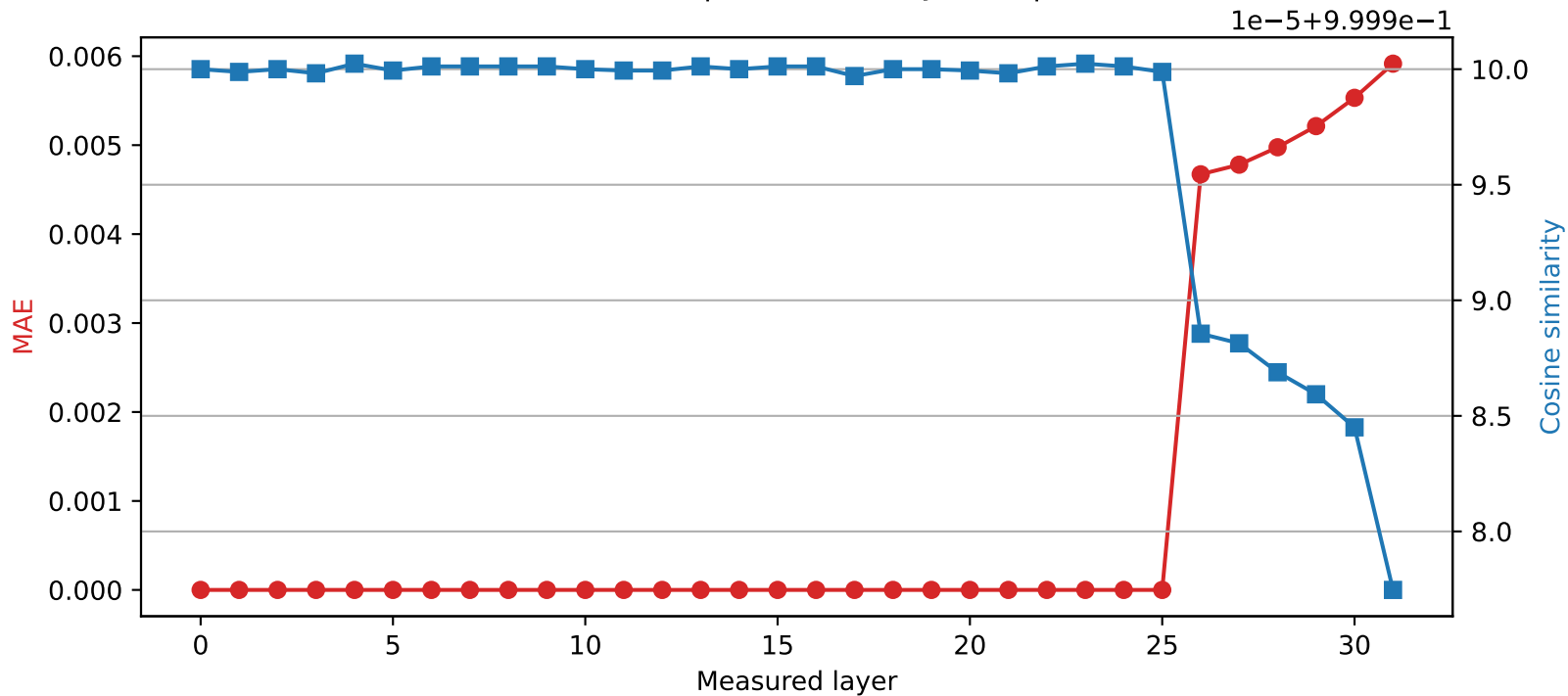
Mistral-7B-Instruct-v0.3 | Quantized layer 25 | float64 \rightarrow int8
