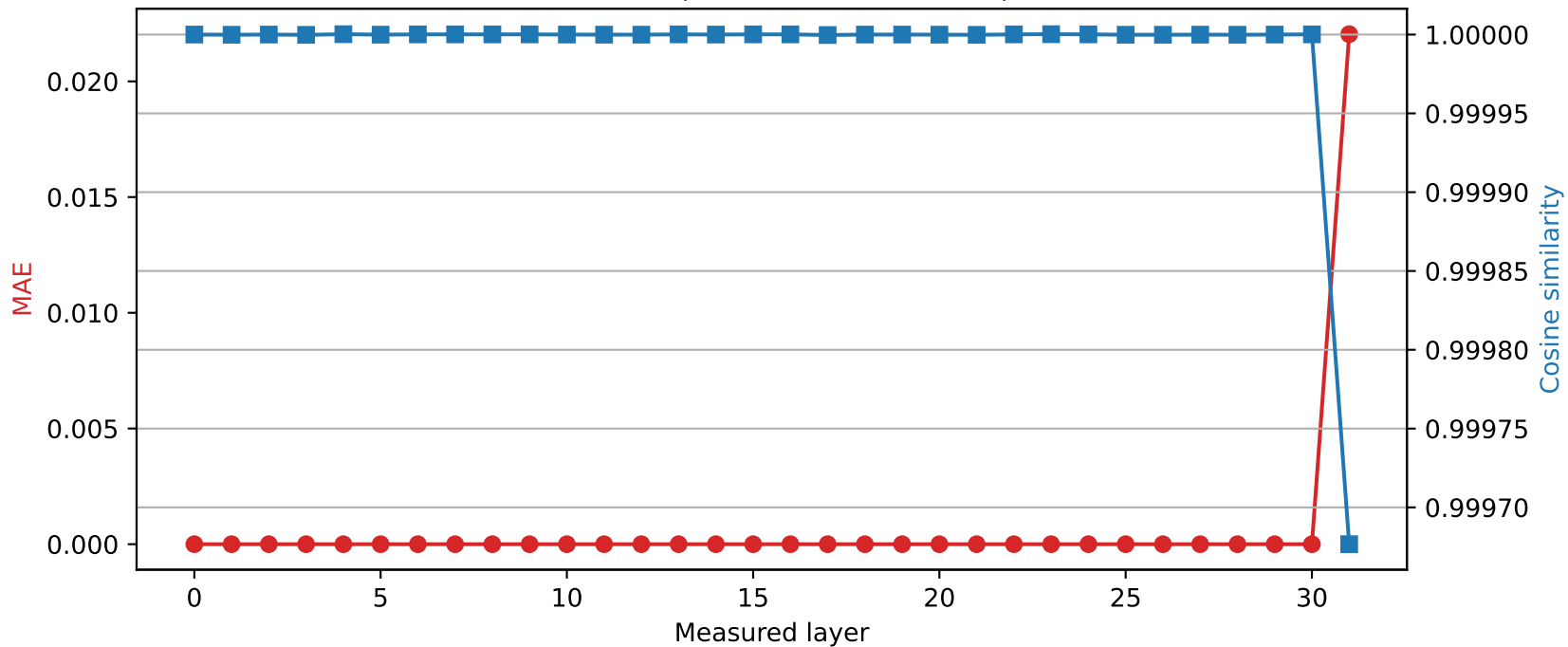
Mistral-7B-Instruct-v0.3 | Quantized layer 30 | float64 → int8
