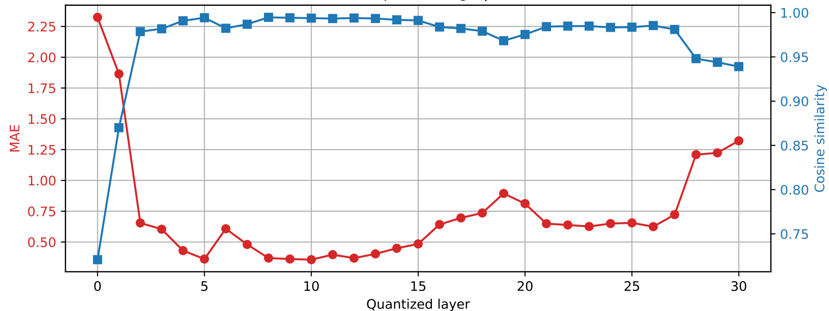
Mistral-7B-Instruct-v0.3 | Prompt 0 Final RMSNorm output damage | float64 \rightarrow int4
