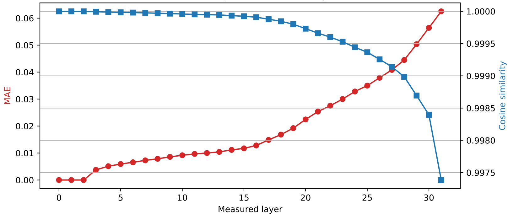
Mistral-7B-Instruct-v0.3 | Quantized layer 2 | float64 → int4
