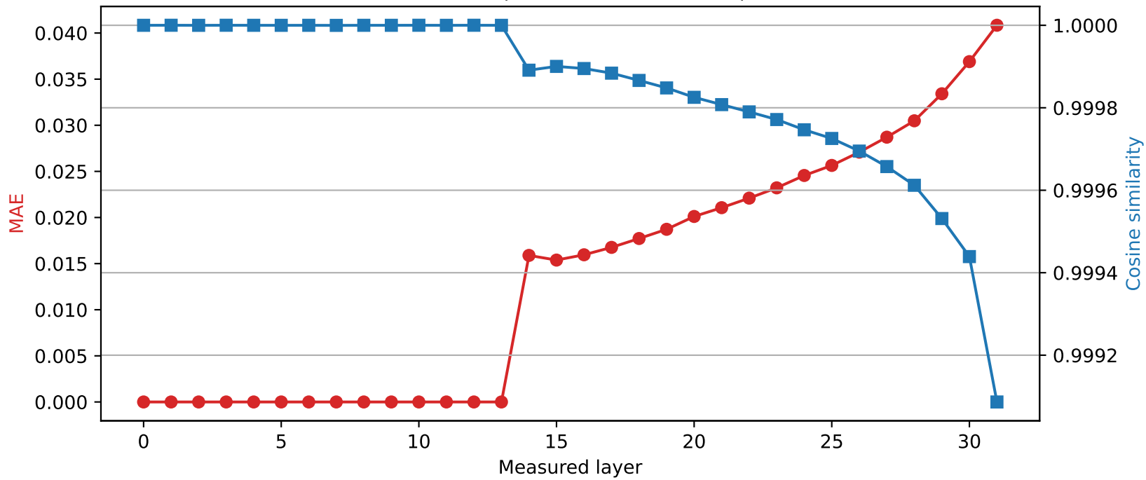
Mistral-7B-Instruct-v0.3 | Quantized layer 13 | float64 \rightarrow int4
