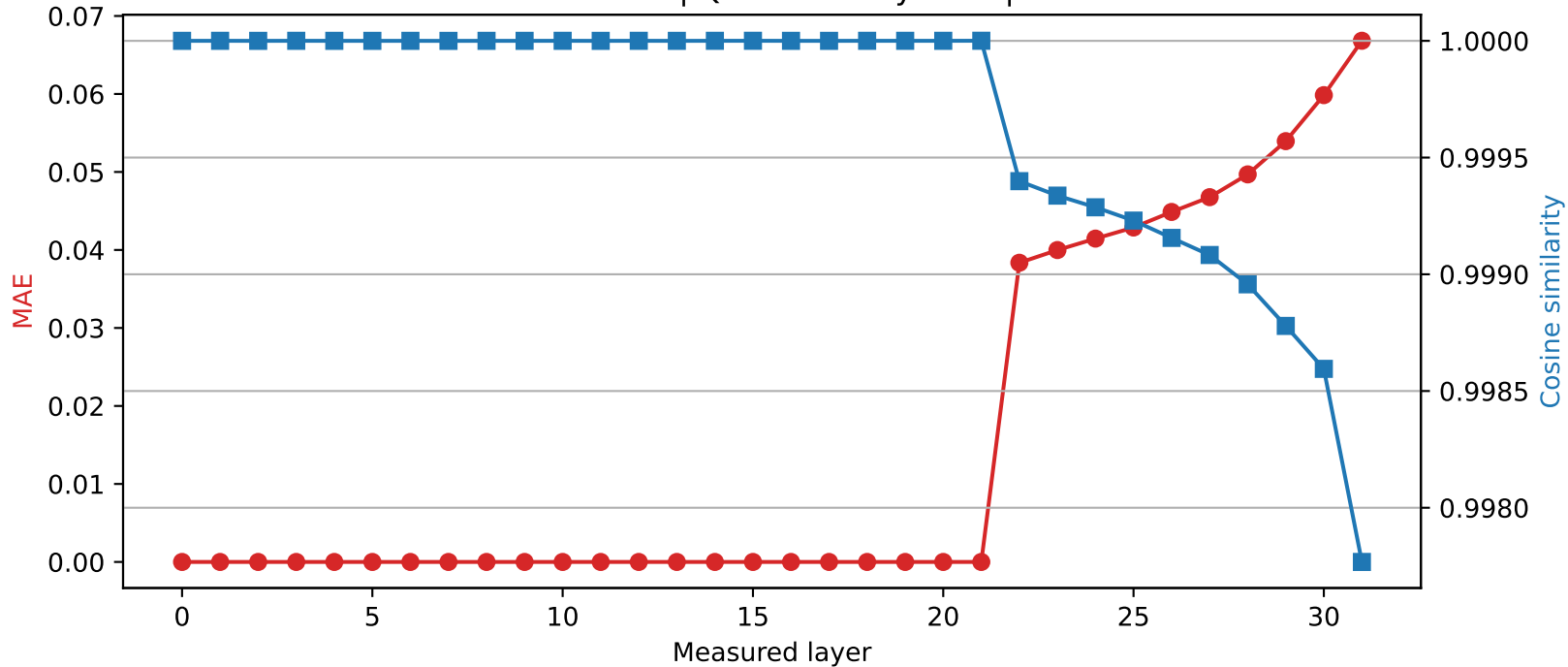
Mistral-7B-Instruct-v0.3 | Quantized layer 21 | float64 \rightarrow int4
