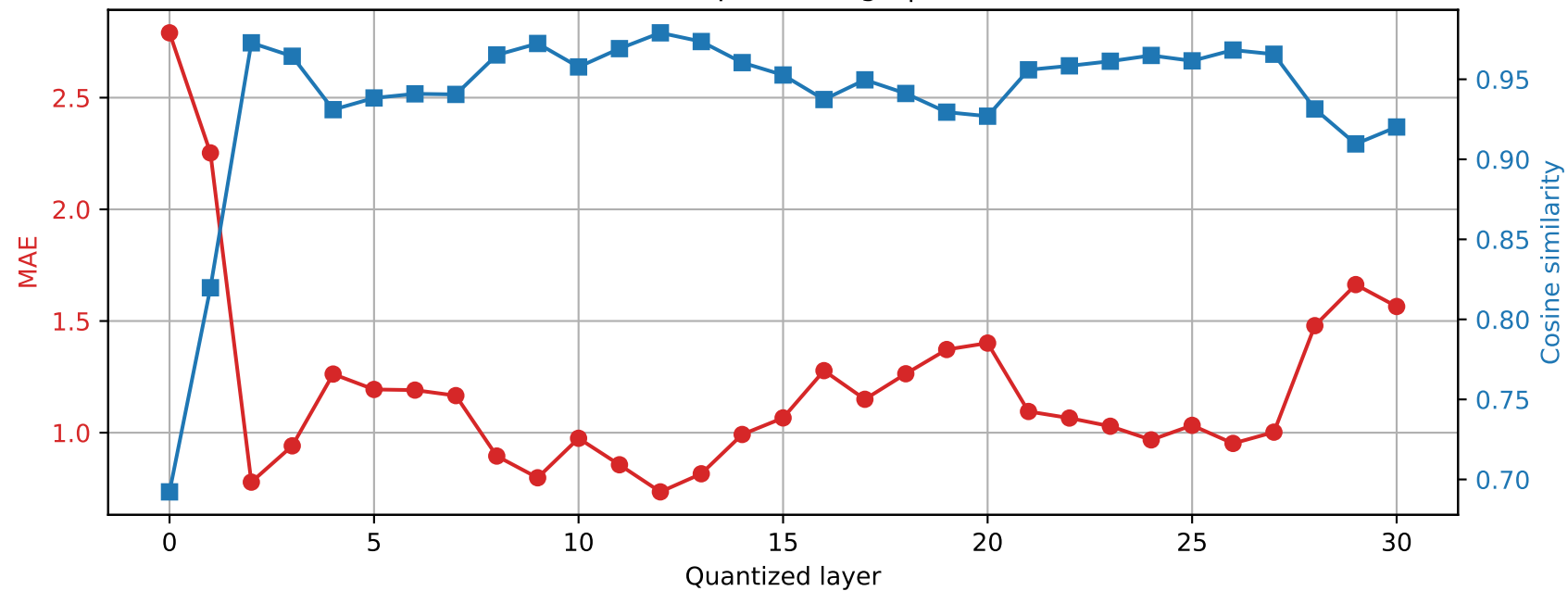
Mistral-7B-Instruct-v0.3 | Prompt 1 Final RMSNorm output damage | float64 → int4
