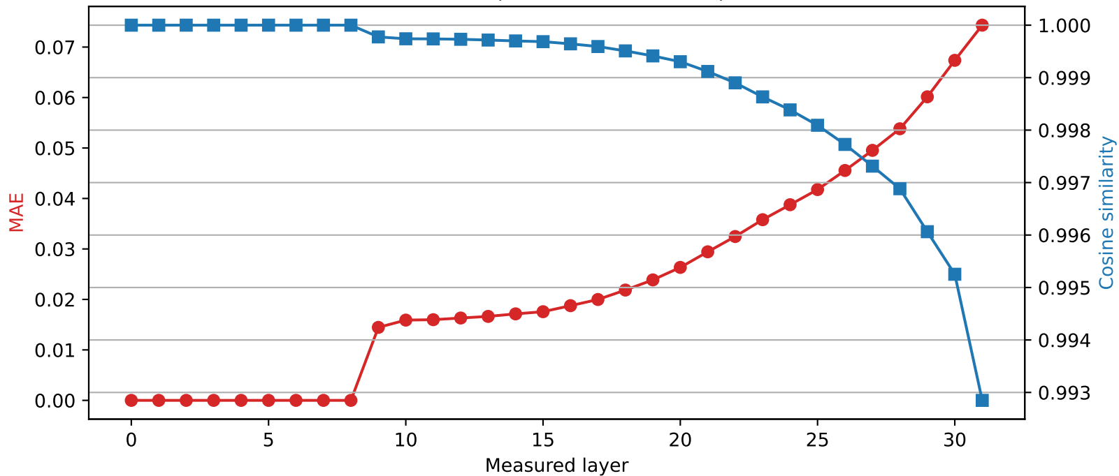
Mistral-7B-Instruct-v0.3 | Quantized layer 8 | float64 → int4
