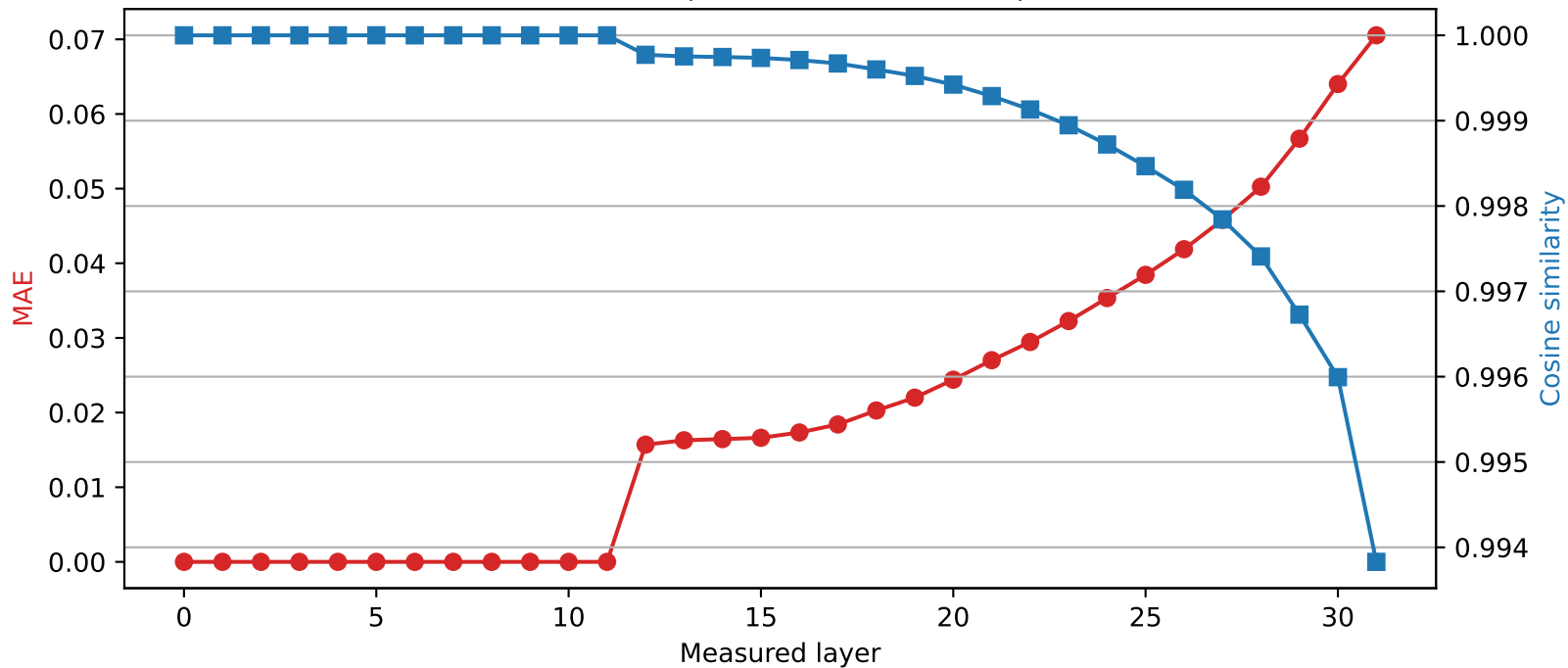
Mistral-7B-Instruct-v0.3 | Quantized layer 11 | float64 → int4
