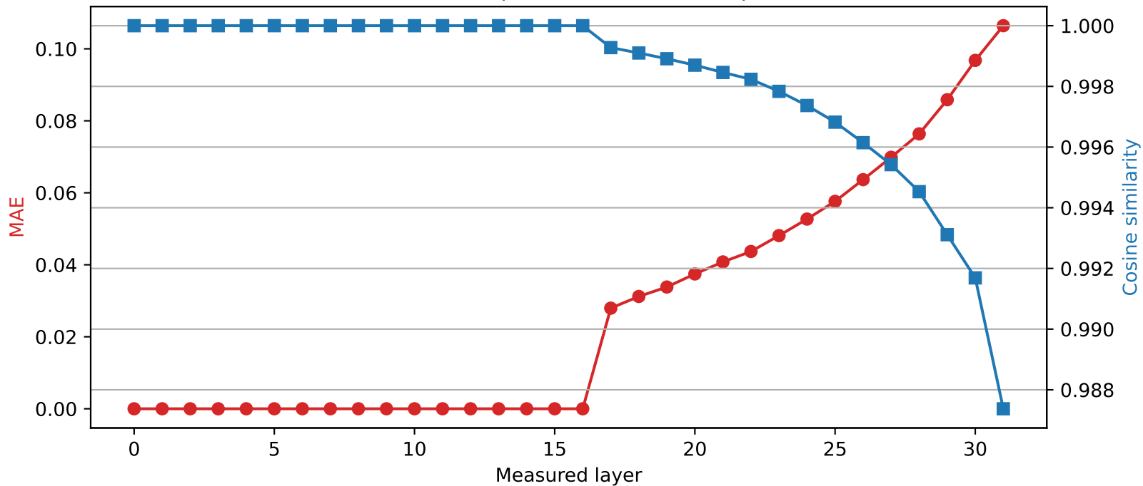
Mistral-7B-Instruct-v0.3 | Quantized layer 16 | float64 → int4
