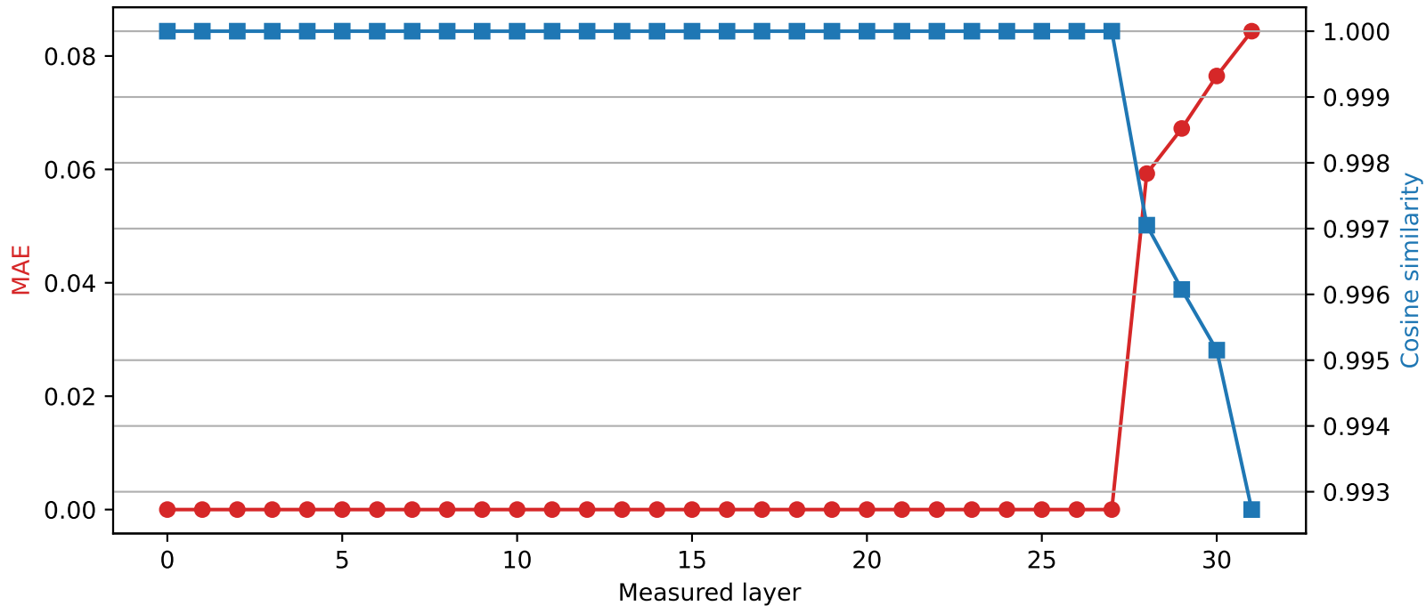
Mistral-7B-Instruct-v0.3 | Quantized layer 27 | float64 → int4
