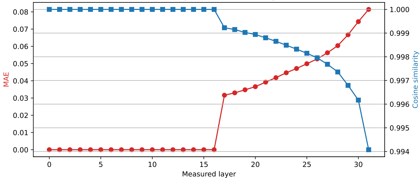
Mistral-7B-Instruct-v0.3 | Quantized layer 16 | float64 \rightarrow int4
