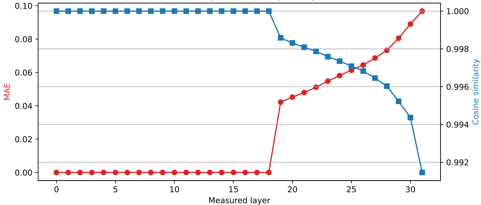
Mistral-7B-Instruct-v0.3 | Quantized layer 18 | float64 → int4
