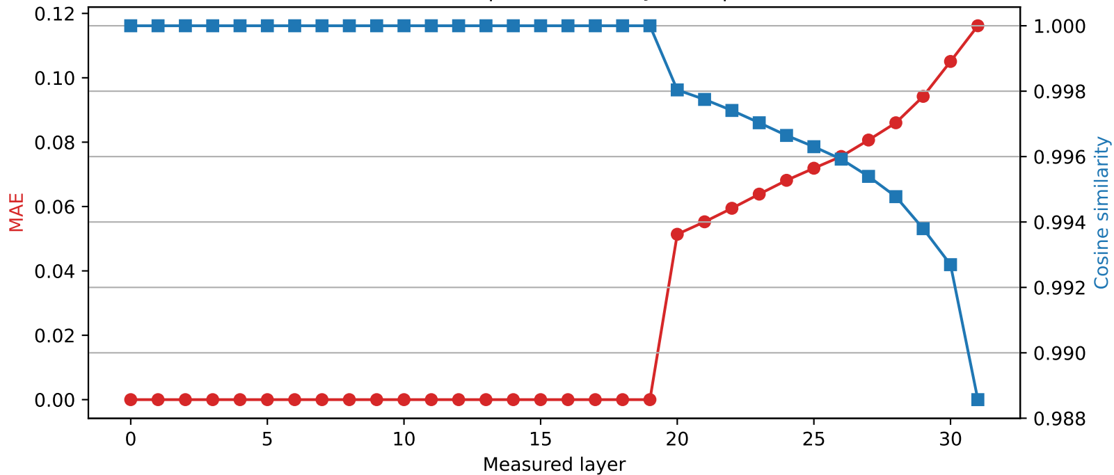
Mistral-7B-Instruct-v0.3 | Quantized layer 19 | float64 \rightarrow int4
