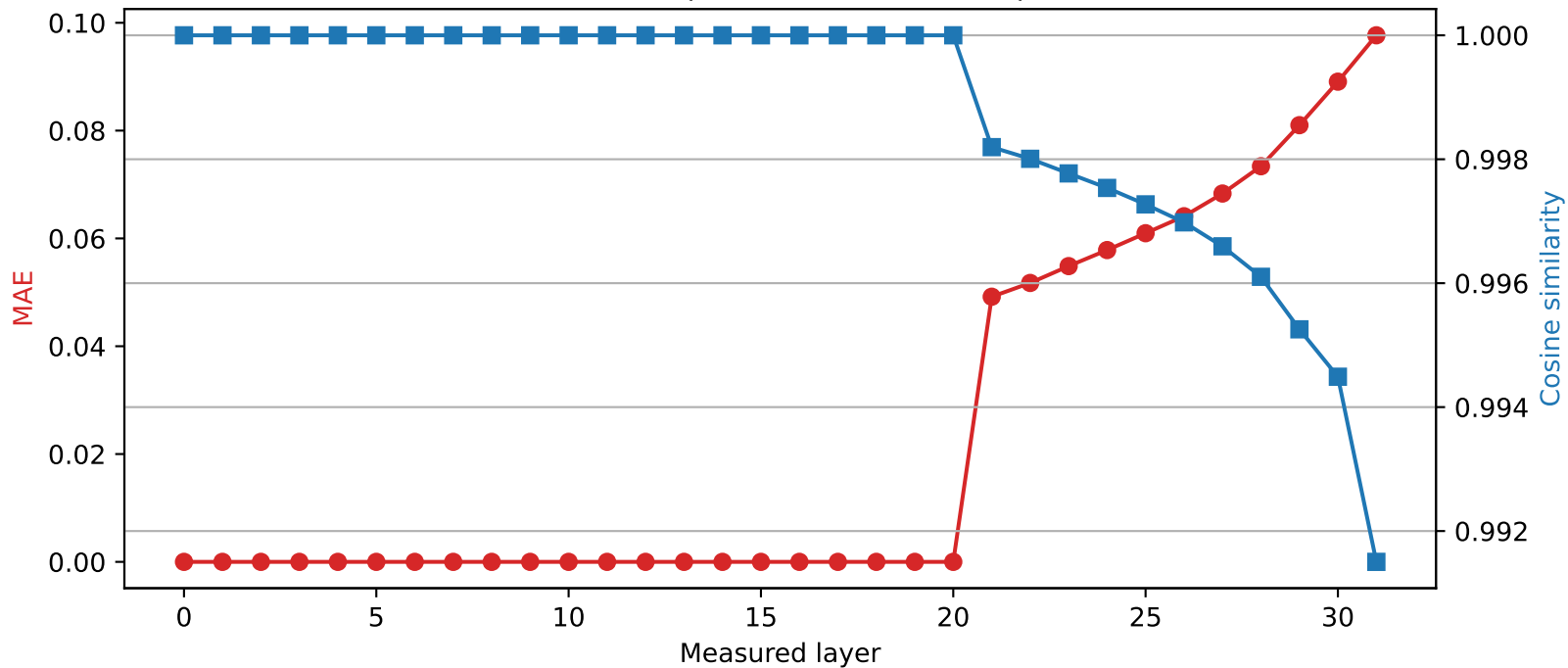
Mistral-7B-Instruct-v0.3 | Quantized layer 20 | float64 \rightarrow int4
