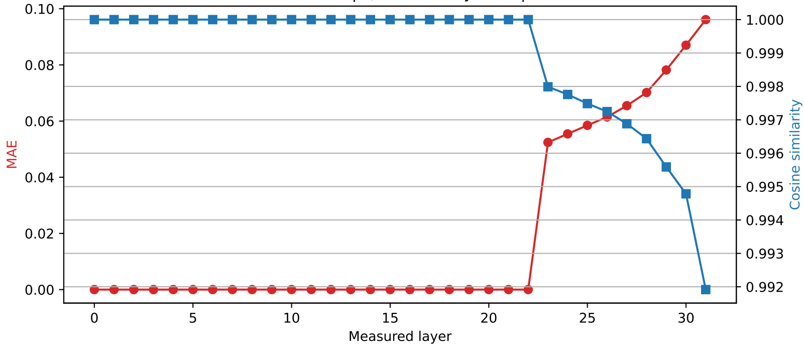
Mistral-7B-Instruct-v0.3 | Quantized layer 22 | float64 \rightarrow int4
