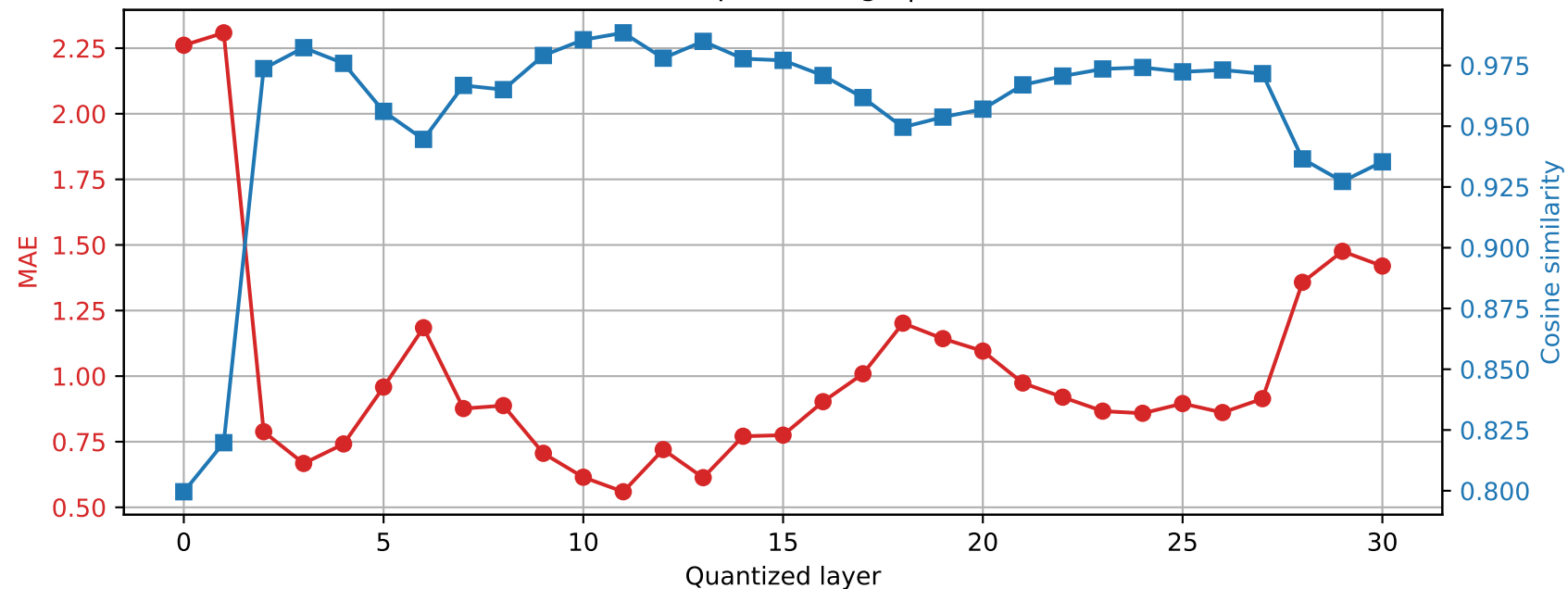
Mistral-7B-Instruct-v0.3 | Prompt 3 Final RMSNorm output damage | float64 → int4
