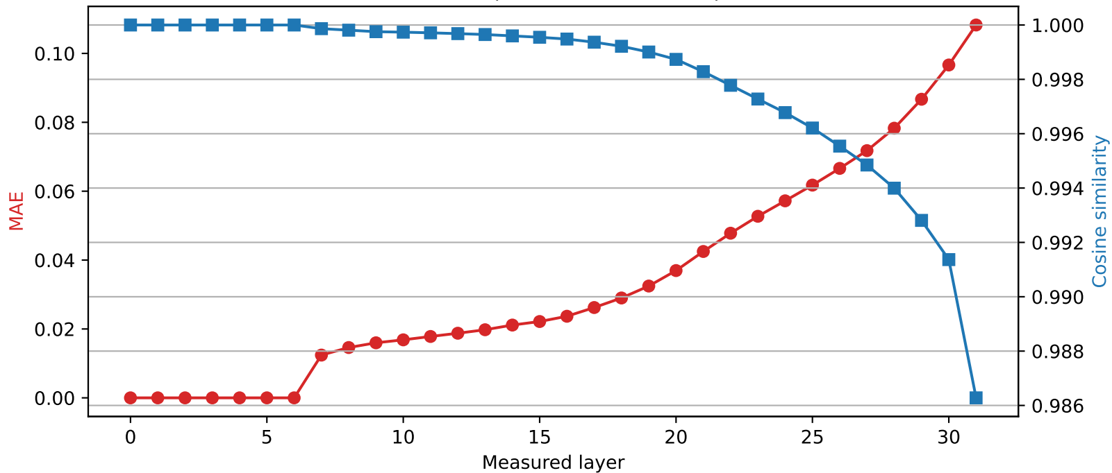
Mistral-7B-Instruct-v0.3 | Quantized layer 6 | float64 → int4
