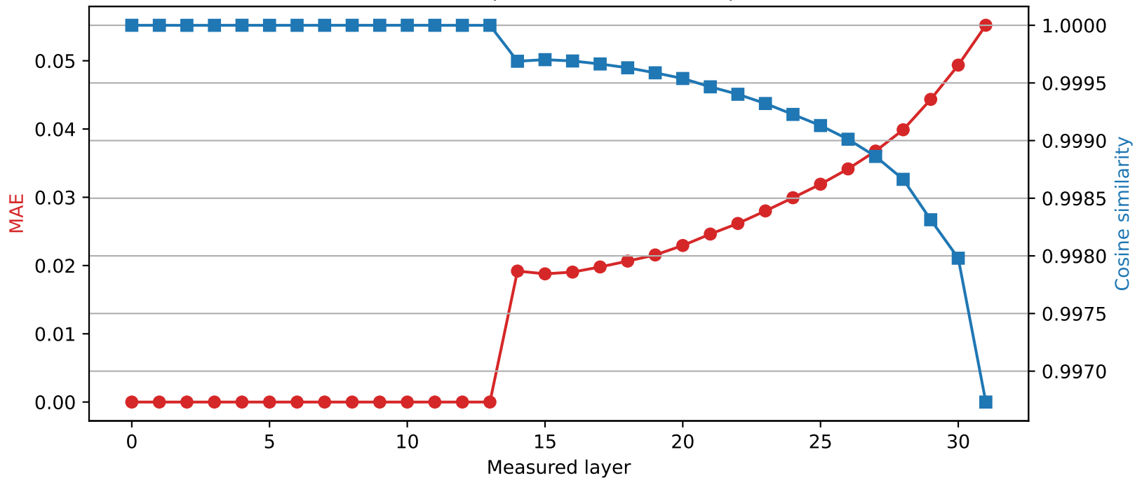
Mistral-7B-Instruct-v0.3 | Quantized layer 13 | float64 → int4
