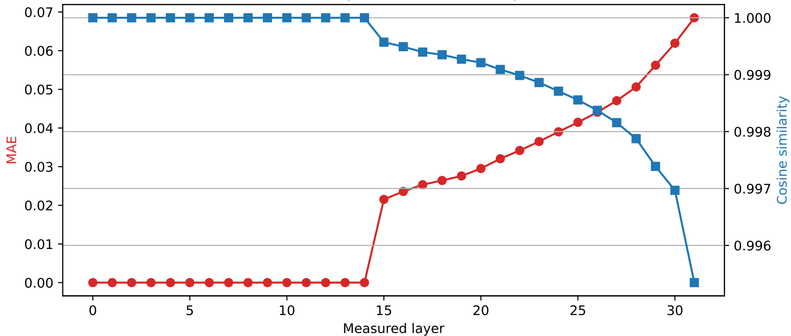
Mistral-7B-Instruct-v0.3 | Quantized layer 14 | float64 \rightarrow int4
