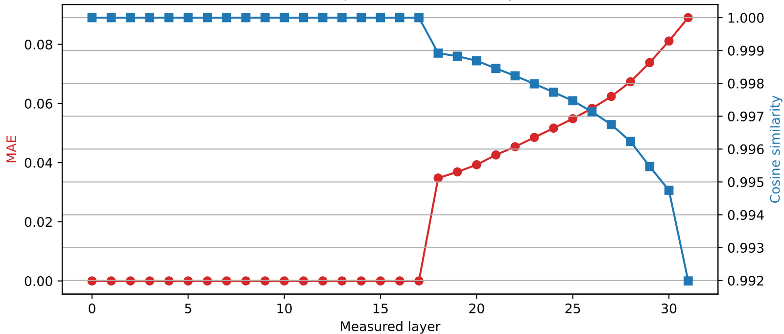
Mistral-7B-Instruct-v0.3 | Quantized layer 17 | float64 \rightarrow int4
