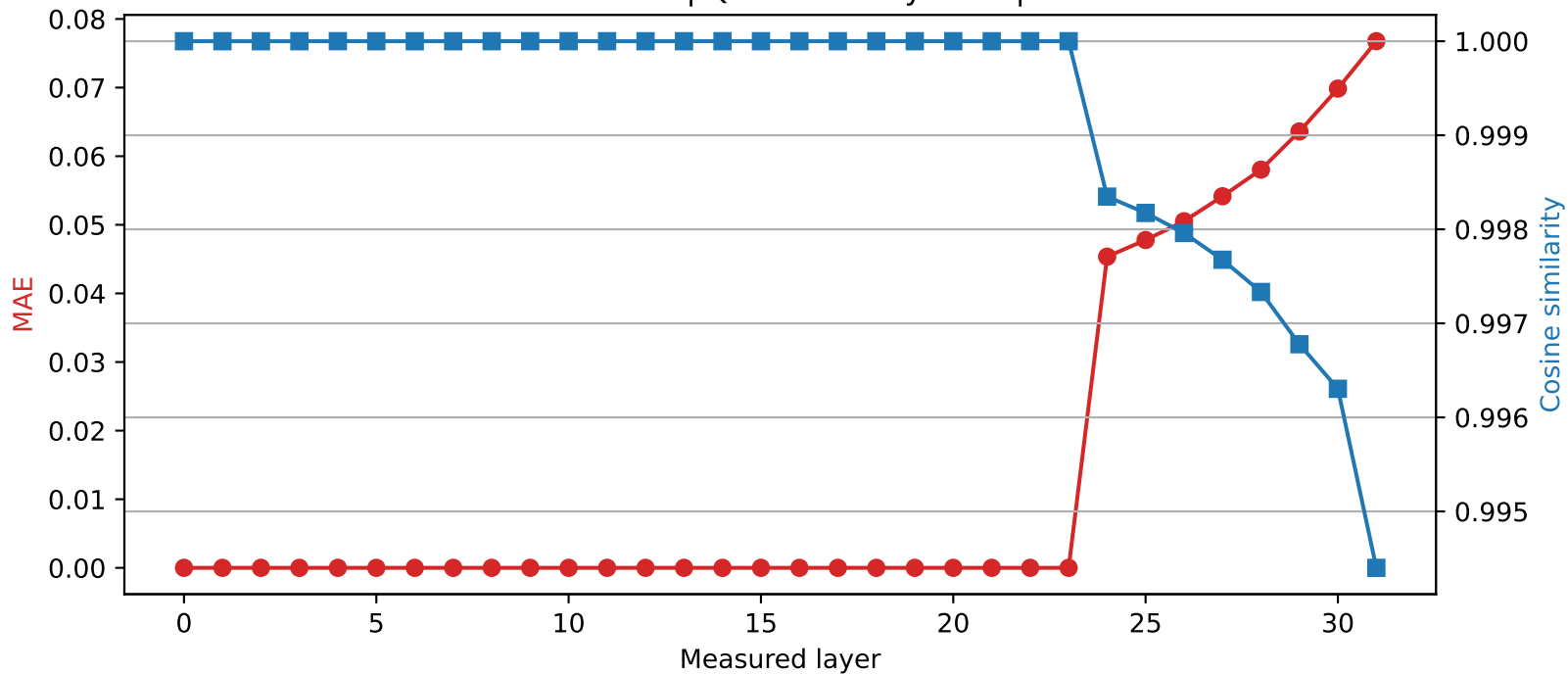
Mistral-7B-Instruct-v0.3 | Quantized layer 23 | float64 \rightarrow int4
