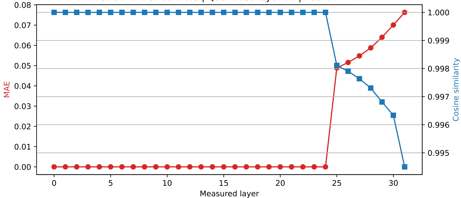
Mistral-7B-Instruct-v0.3 | Quantized layer 24 | float64 → int4
