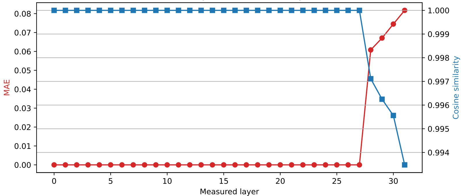
Mistral-7B-Instruct-v0.3 | Quantized layer 27 | float64 \rightarrow int4
