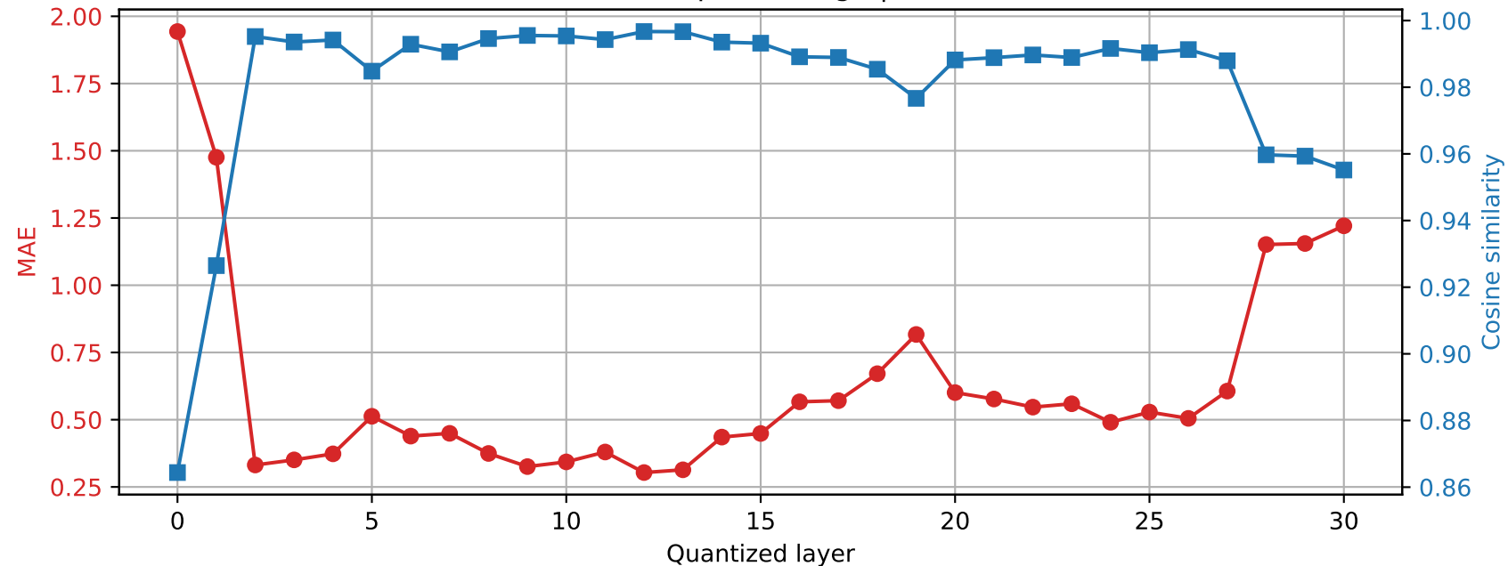
Mistral-7B-Instruct-v0.3 | Prompt 4 Final RMSNorm output damage | float64 \rightarrow int4
