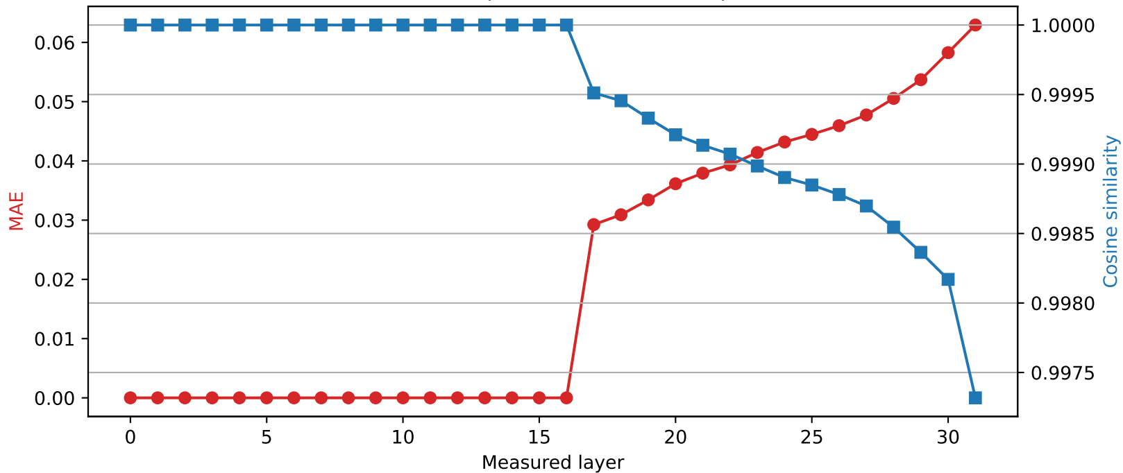
Mistral-7B-Instruct-v0.3 | Quantized layer 16 | float64 \rightarrow int4
