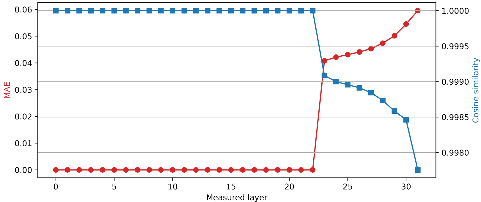
Mistral-7B-Instruct-v0.3 | Quantized layer 22 | float64 → int4
