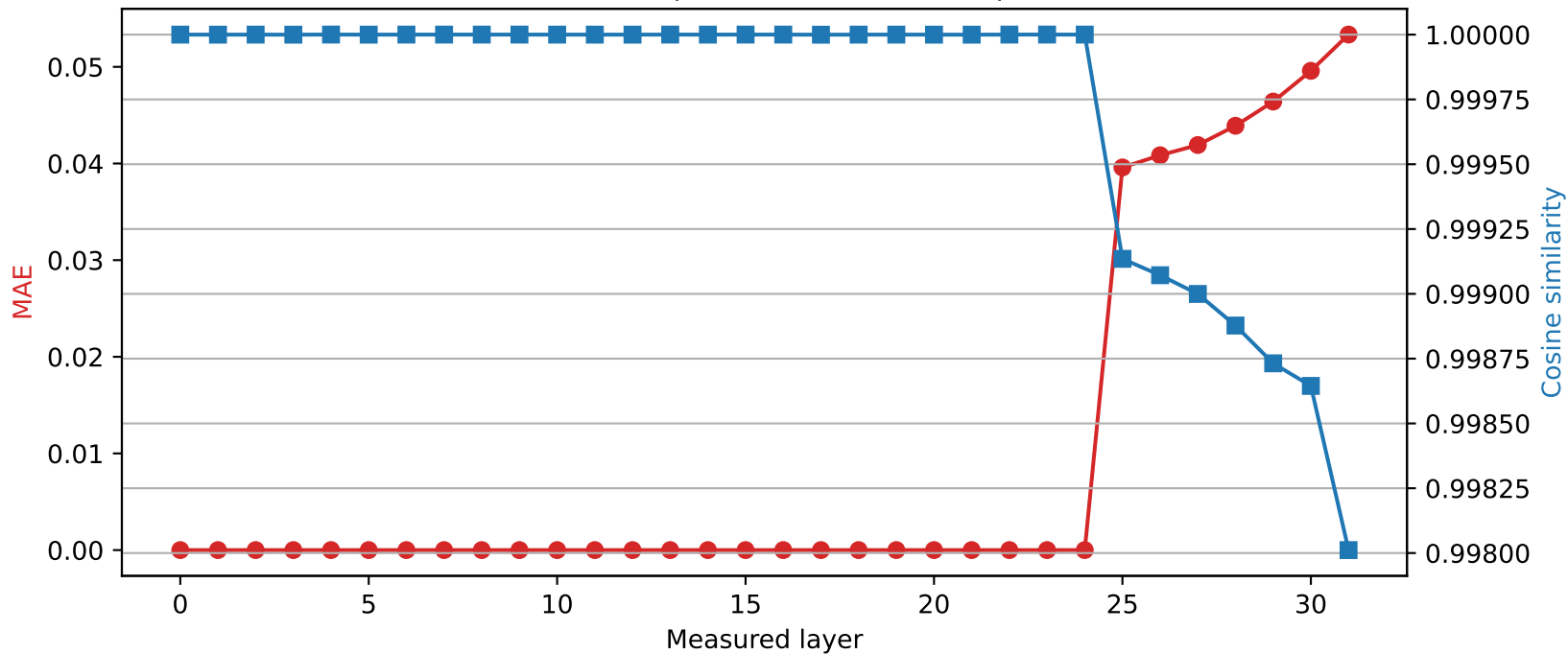
Mistral-7B-Instruct-v0.3 | Quantized layer 24 | float64 \rightarrow int4
