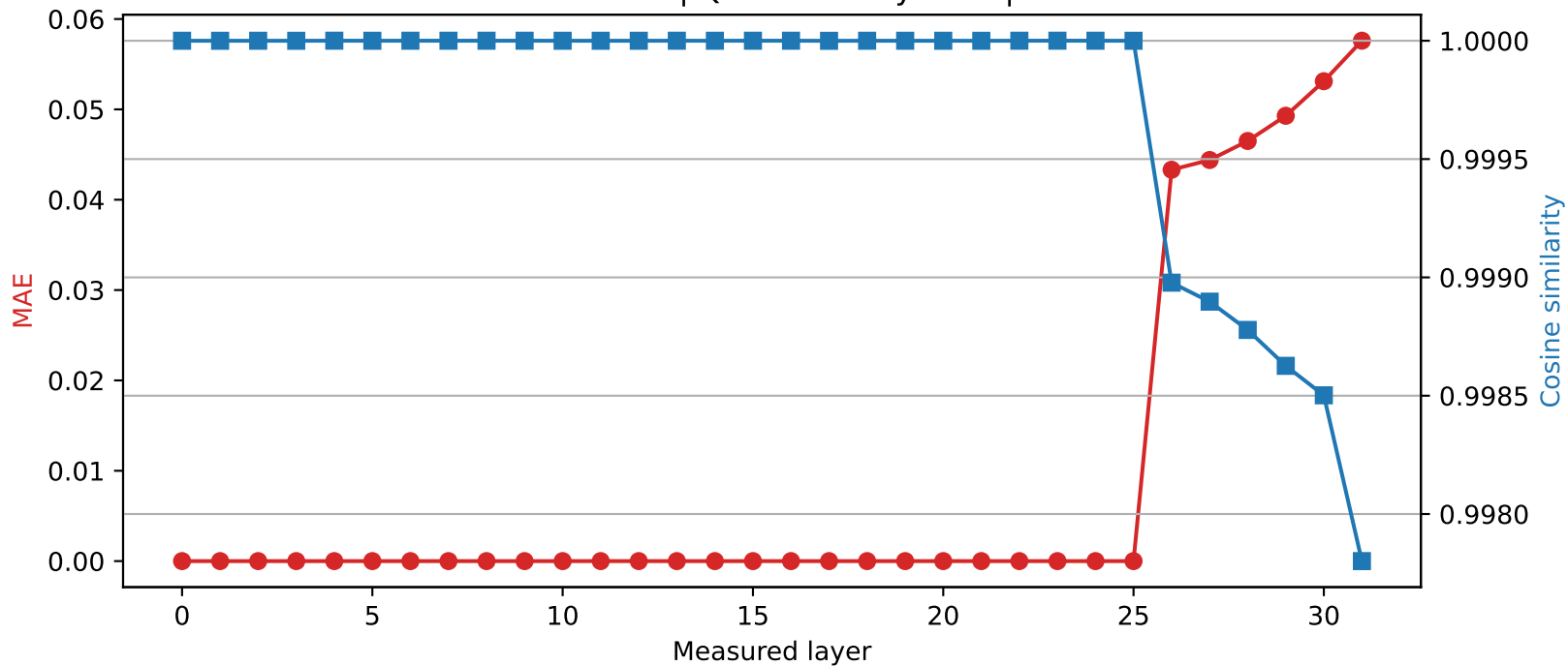
Mistral-7B-Instruct-v0.3 | Quantized layer 25 | float64 \rightarrow int4
