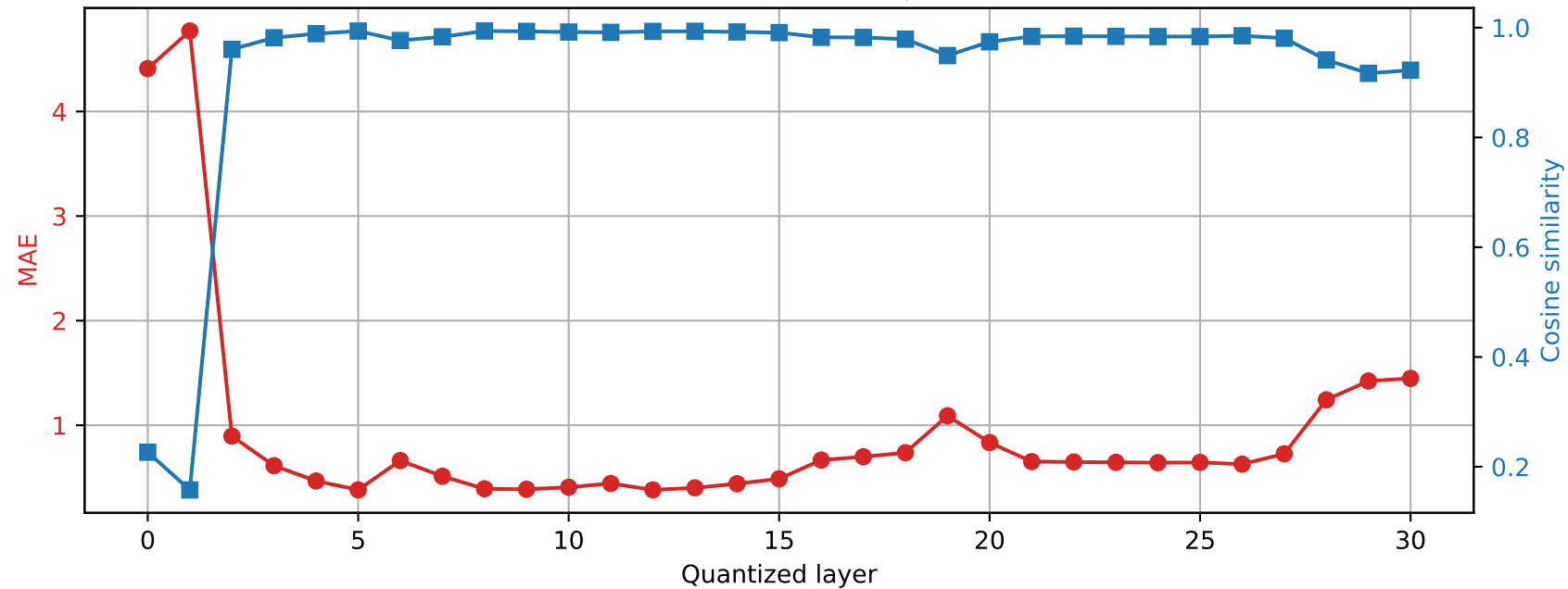
Mistral-7B-Instruct-v0.3 | Prompt 0 Final RMSNorm output damage | float64 → int2
