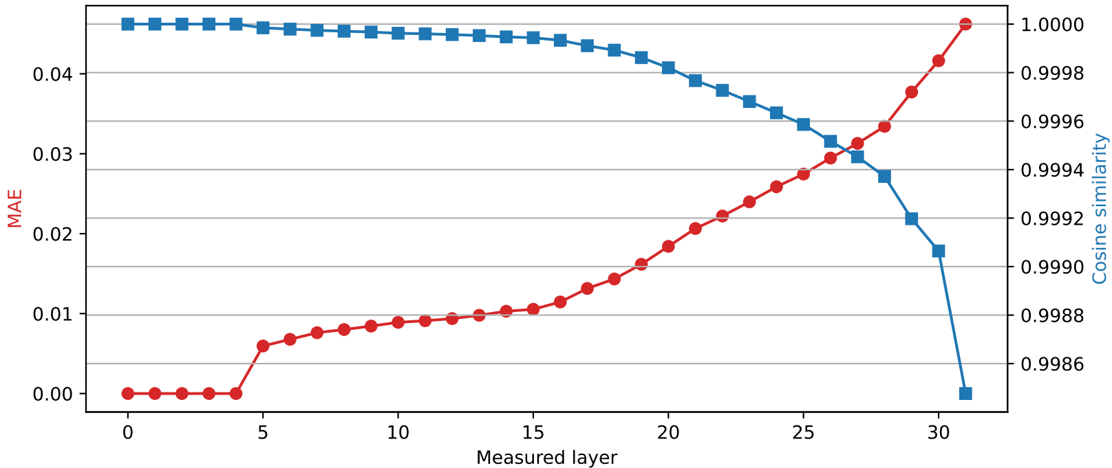
Mistral-7B-Instruct-v0.3 | Quantized layer 4 | float64 → int2
