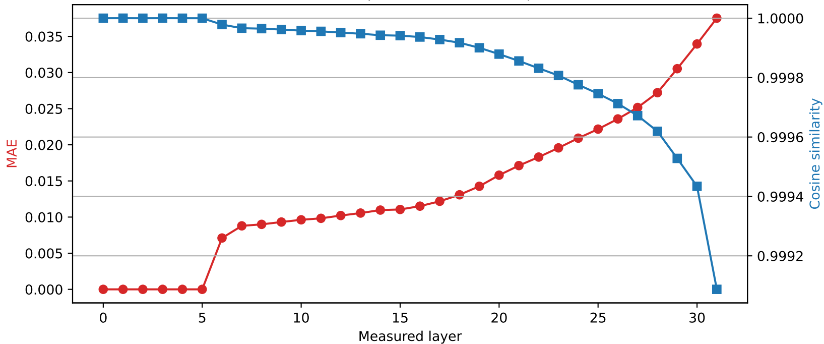
Mistral-7B-Instruct-v0.3 | Quantized layer 5 | float64 \rightarrow int2
