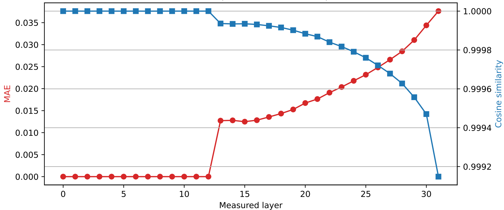
Mistral-7B-Instruct-v0.3 | Quantized layer 12 | float64 \rightarrow int2
