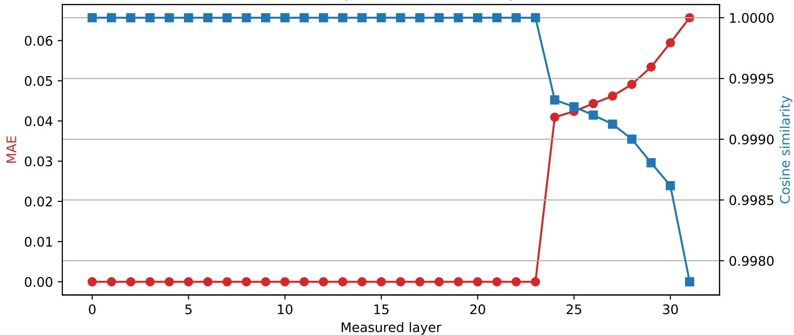
Mistral-7B-Instruct-v0.3 | Quantized layer 23 | float64 \rightarrow int2
