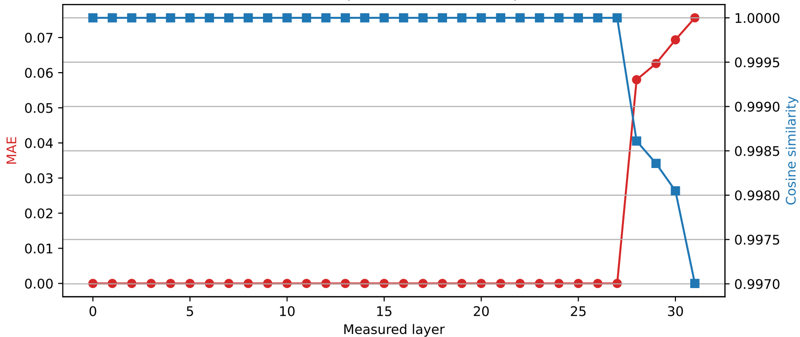
Mistral-7B-Instruct-v0.3 | Quantized layer 27 | float64 \rightarrow int2
