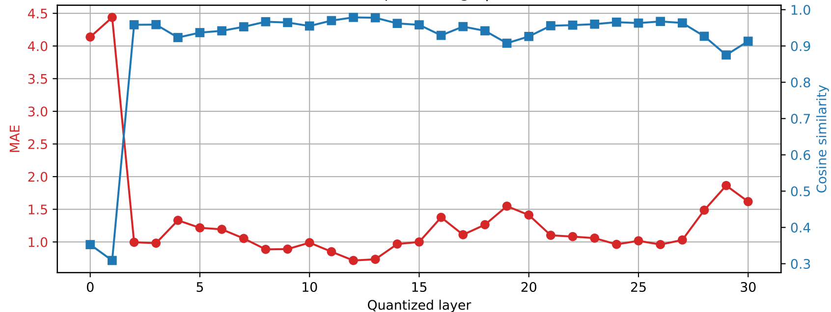
Mistral-7B-Instruct-v0.3 | Prompt 1 Final RMSNorm output damage | float64 \rightarrow int2
