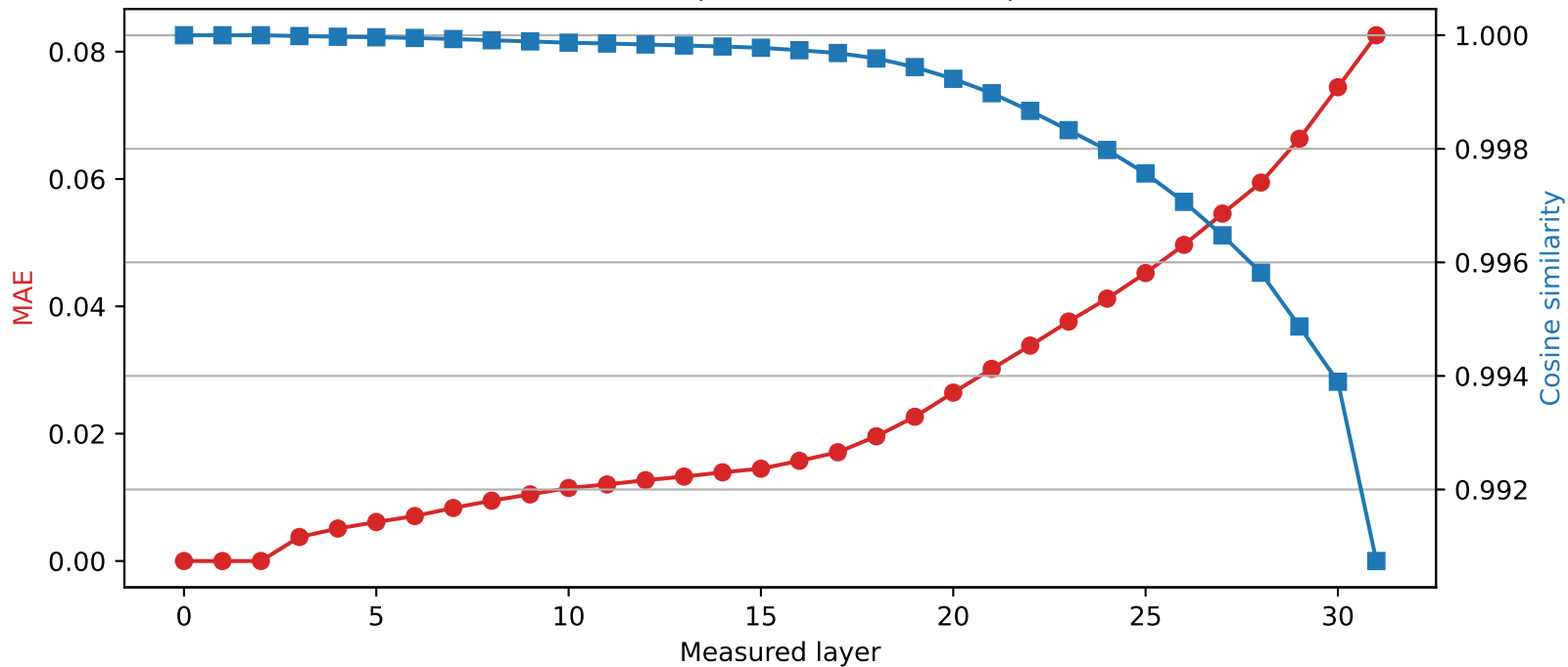
Mistral-7B-Instruct-v0.3 | Quantized layer 2 | float64 → int2
