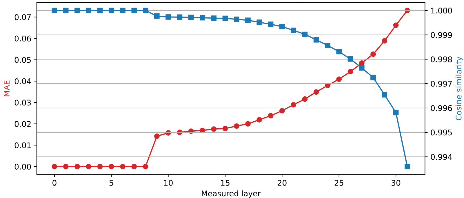
Mistral-7B-Instruct-v0.3 | Quantized layer 8 | float64 → int2
