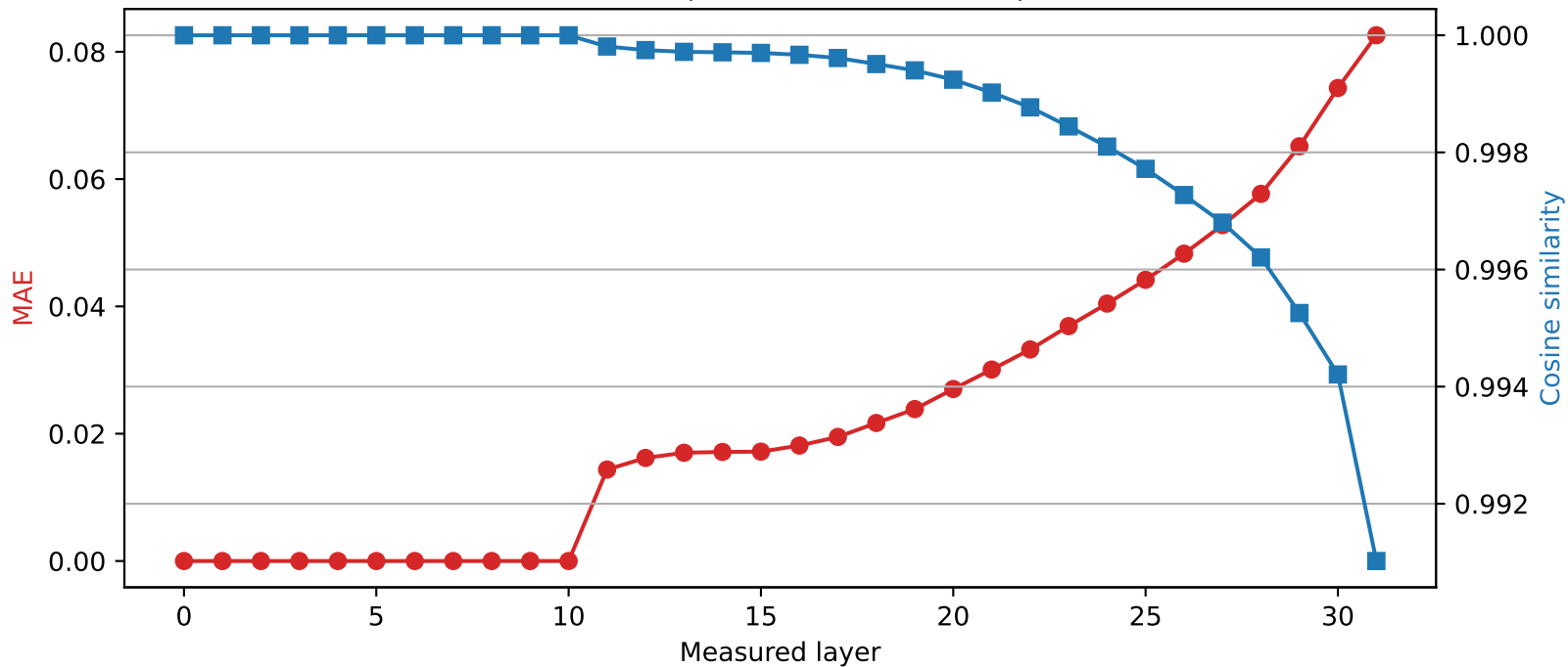
Mistral-7B-Instruct-v0.3 | Quantized layer 10 | float64 \rightarrow int2
