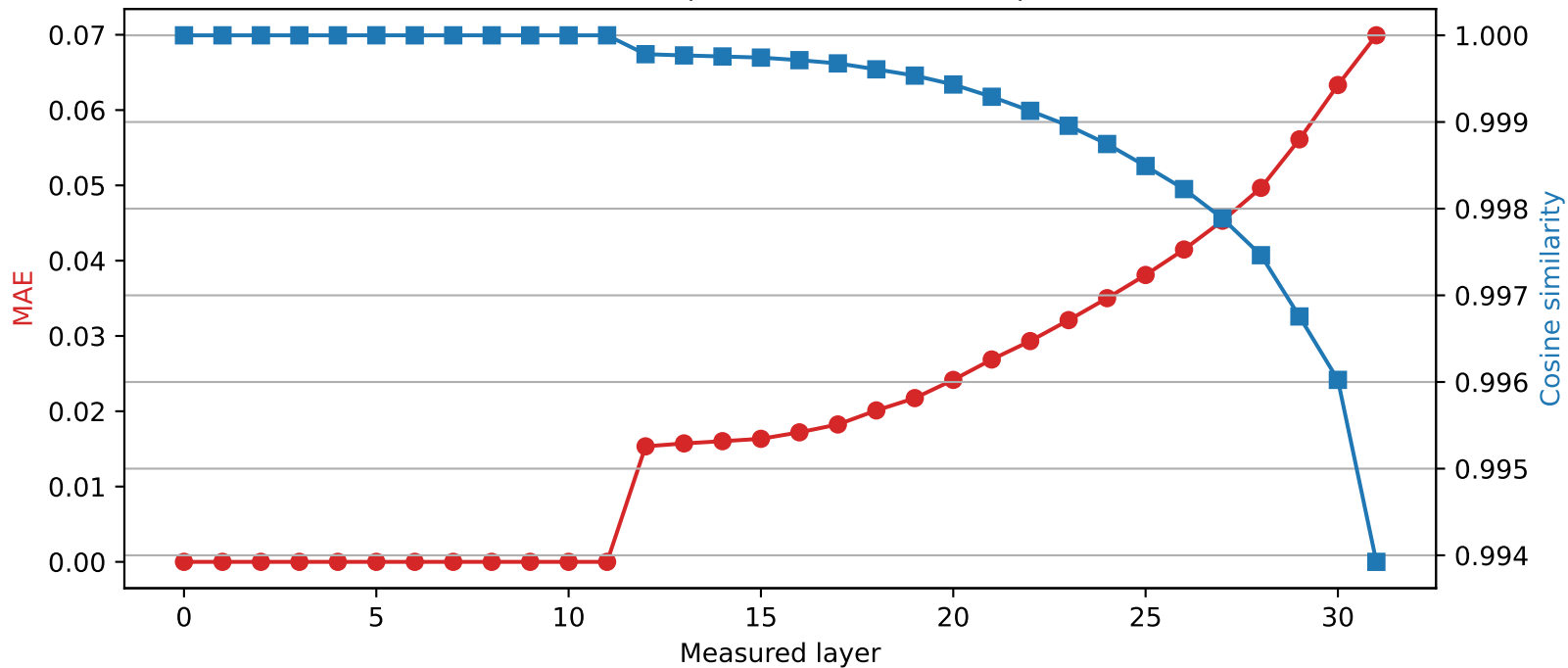
Mistral-7B-Instruct-v0.3 | Quantized layer 11 | float64 → int2
